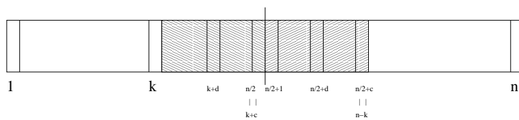
Figure 2: distinguished regions and places in a permutation
