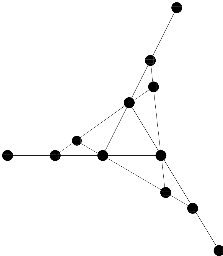
Figure 1: a set G with D(G) = 2
