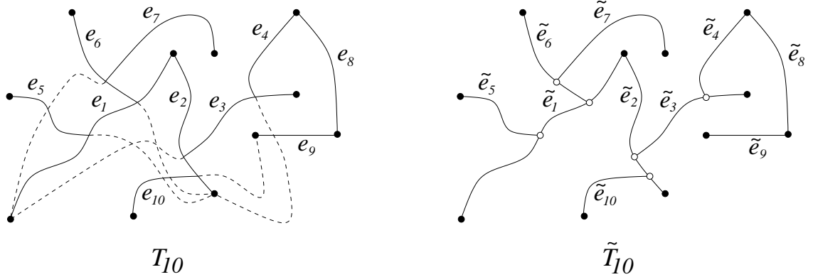
Figure 2. Constructing \tilde{T}_{10} from T_{10}
