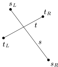
Figure 1: Intersection of the segments s and t .
